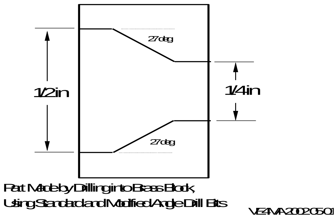
Figure 4 47 GHz Feedhorn
