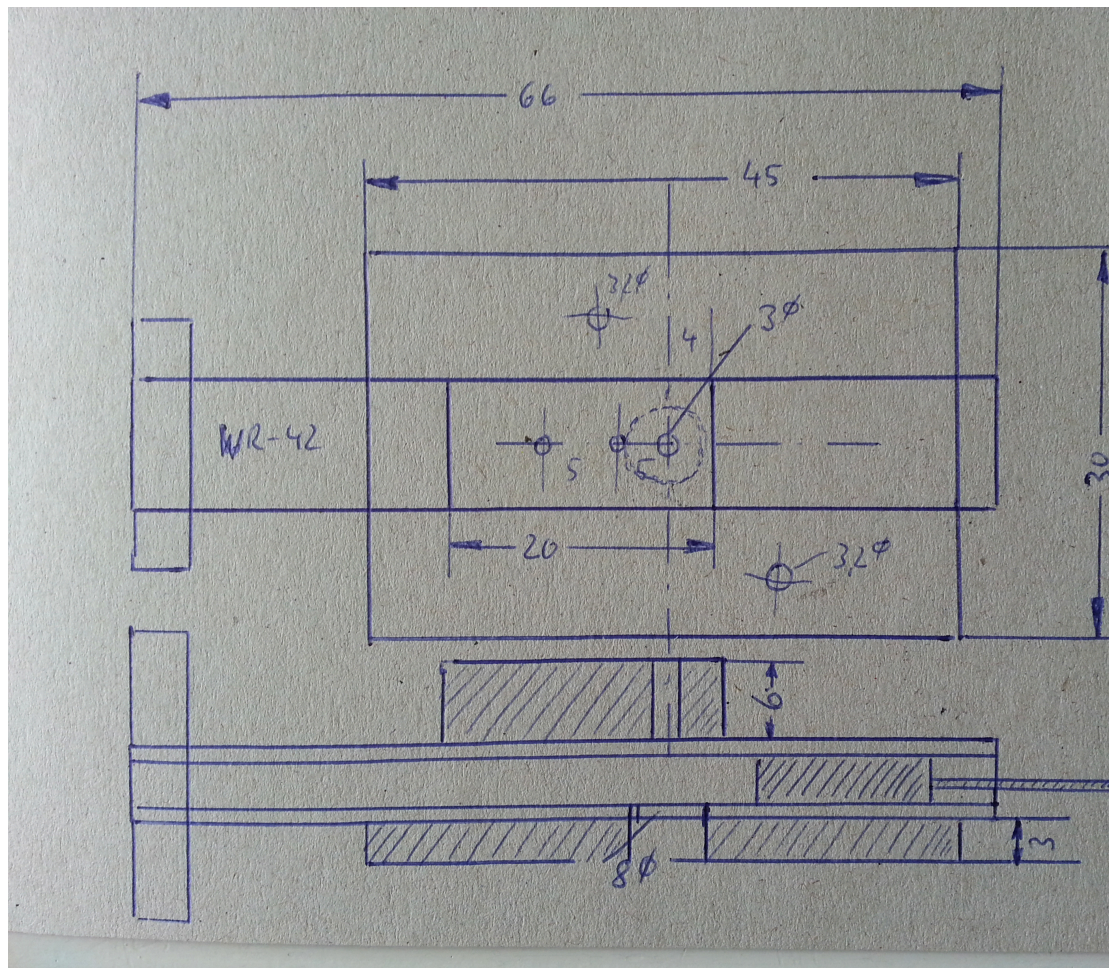
Mechanical dimension of the tested 24 GHz WG transition for RW1127 tubes
